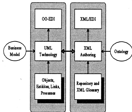
Figure 3: Coupling OO-EDI and XML/EDI
