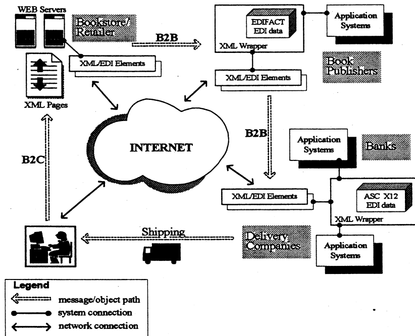
Figure 4: A XML/EDI framework for book enterprises
